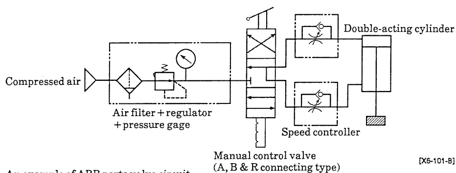
Fig. 2. An example of ABR ports valve circuit
